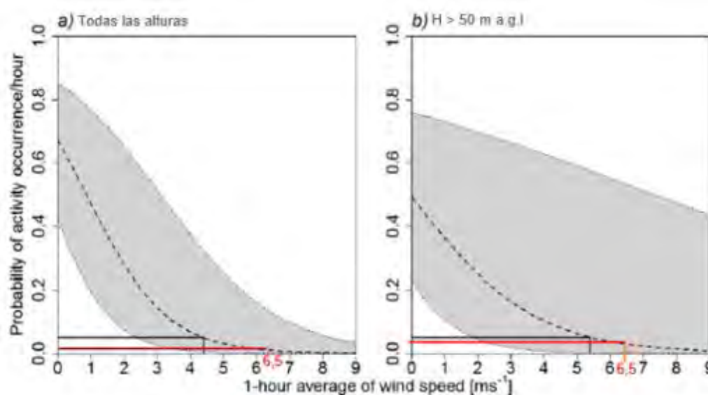
Figura 53. Mitigating the negative impacts of tall wind turbines on bats: Vertical activity profiles and relationships to wind speed. (Willing, S.D. 2018)
