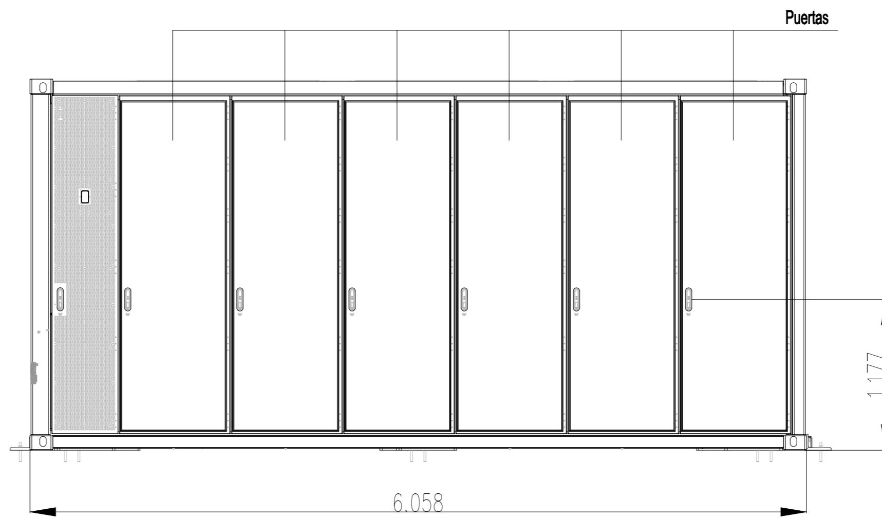
Vista Frontal
